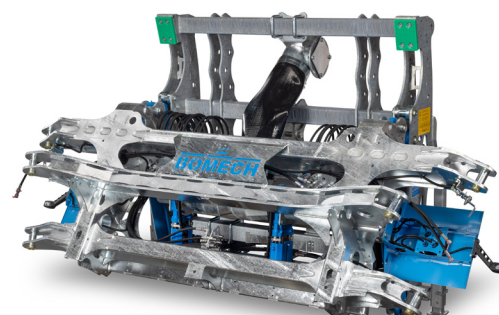
Heavy Construction frame (HC)
